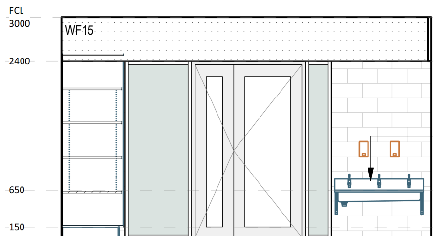
4 ELEVATION DETAIL 60-015 1 : 50
