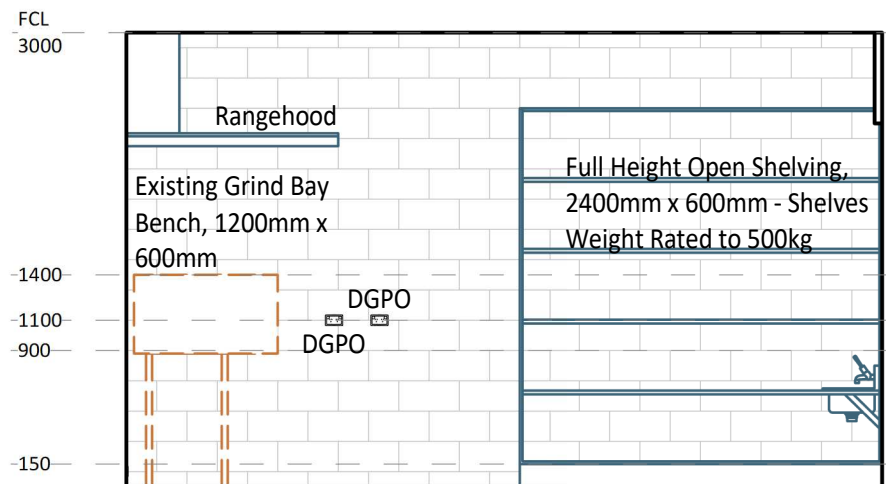
3 ELEVATION DETAIL 60-015 1 : 50
