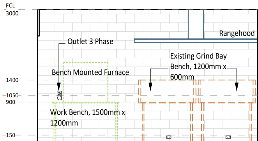
2 ELEVATION DETAIL 60-015 1 : 50
